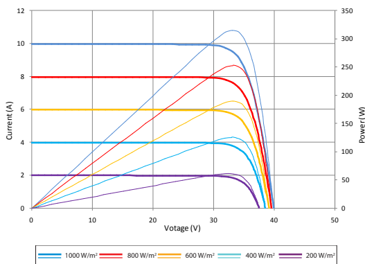
Current-Voltage & Power-Voltage Curve (315S)
